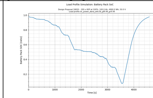
SoC(t) diagram with 2 runs of the WLTP profile + recharging at 6C
